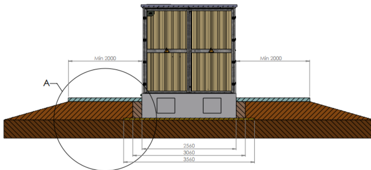
VISTA FRONTAL
